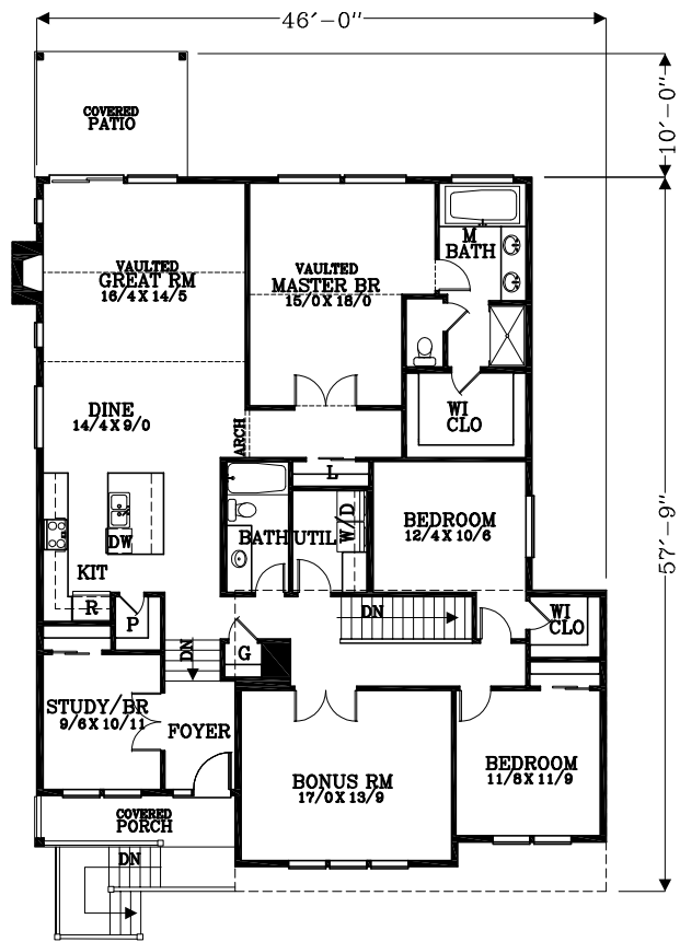
MAIN FLOOR PLAN 2,248 SQUARE FEET 2,248 TOTAL SQUARE FEET
